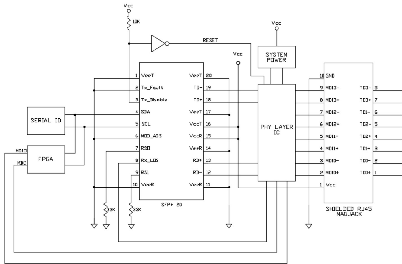
Figure 2. Block diagram
