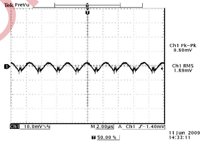
VRP4-C2E1A0 12Vdc input, VID=0x52, Iout=20A, PSI#=0
