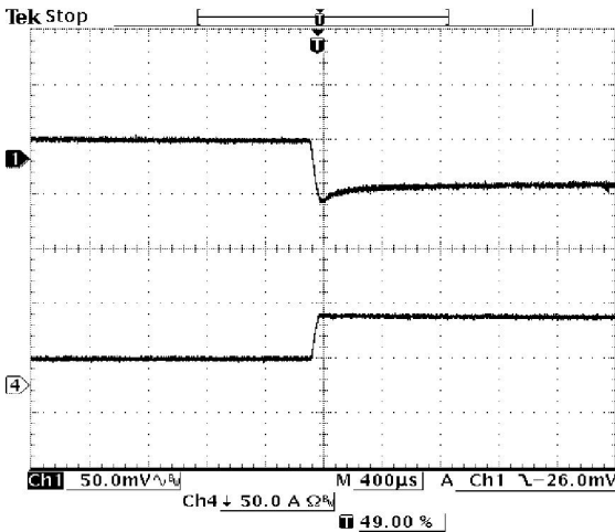
VRP4-C0E1A0 VID=0x52 25A-75A Load Transients at Vin=12V
