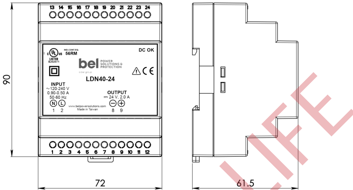
Figure 1. Mechanical Drawing
